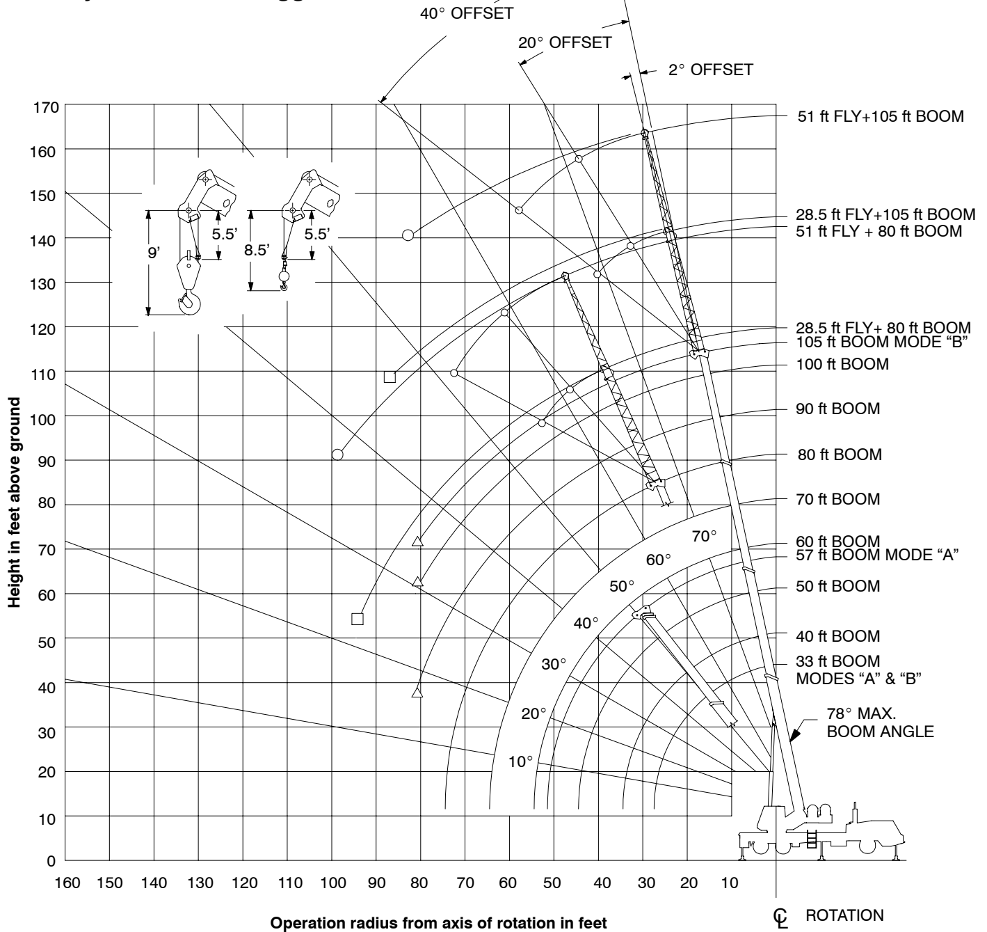
4,700 lb Counterweight
