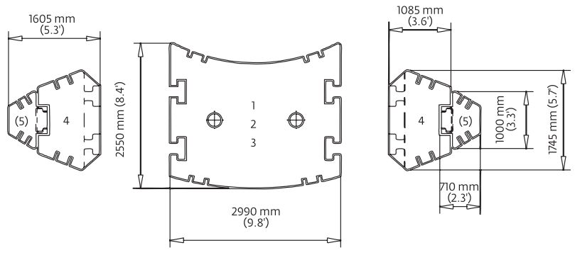
Counterweight Configuration kg (lb)
